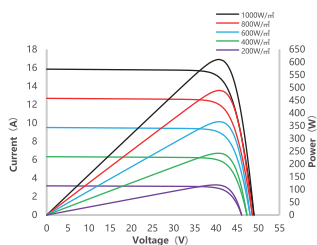
I-V/P-V Curve at Different Irradiation SSA-66HD-610N
