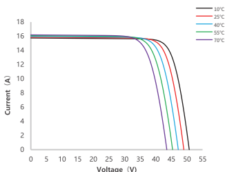
I-V Curve at Different Temperature SSA-66HD-610N
