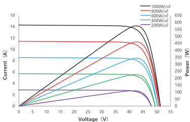
I-V/P-V Curve at Different Irradiation SS8-72HD-575N
