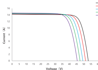
I-V Curve at Different Temperature SS8-72HD-575N
