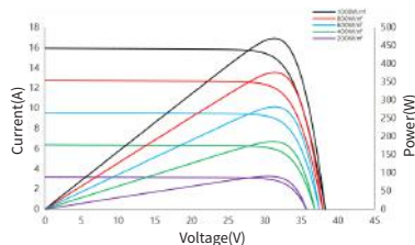
I-V/P-V Curve at Different Irradiation SSA-54HD-495N
