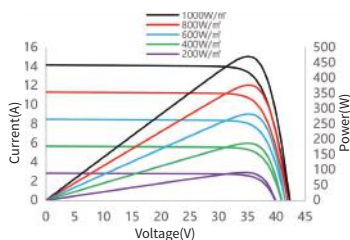
I-V/P-V Curve at Different Irradiation SS8-60HD-470N
