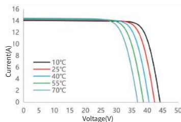
I-V Curve at Different Temperature SS8-60HD-470N
