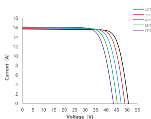
I-V Curve at Different Temperature SSA-66HD-610N
