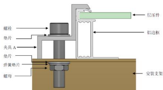
侧边压块
